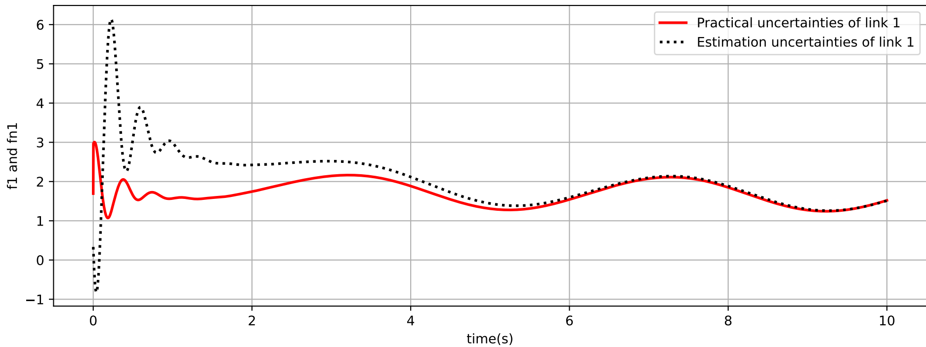
Disturbance Estimation Performance ( S=3 , S1=1 , m=5 )
